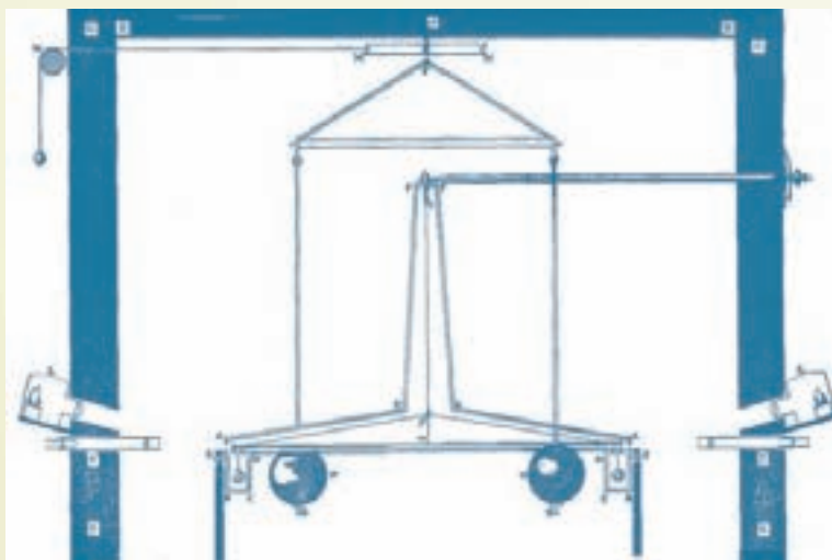
Cavendish' apparatus
